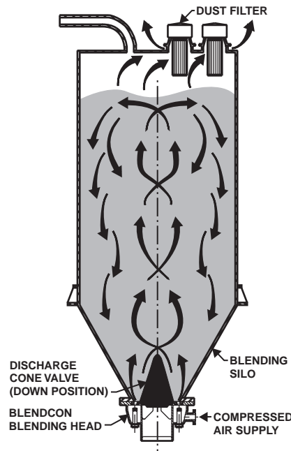
Batch Blending
