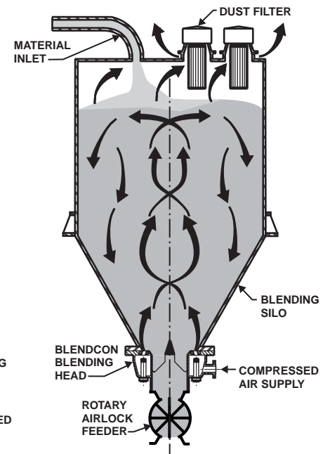
Continuous Blending
